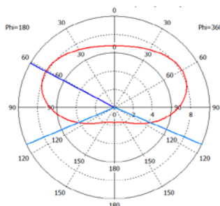
E-plane 3/8 λ dipole to mast spacing
