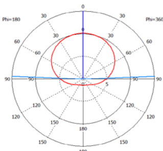
E-plane 1/4 λ dipole to mast spacing
